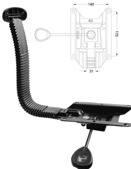
Lever A for seat height adjustment
