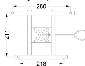
Lever for Seat height adjustment
